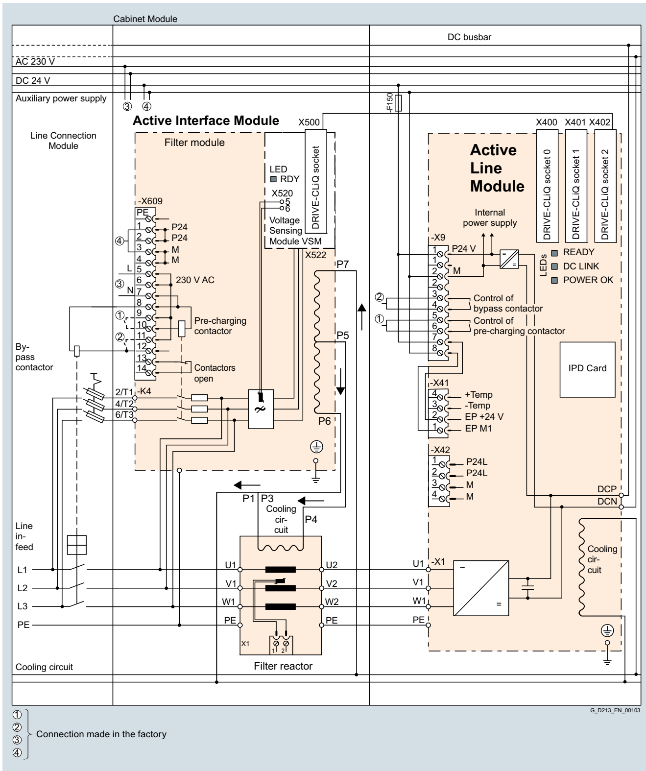
Connection example for the Active Line Connection Module, liquid-cooled
